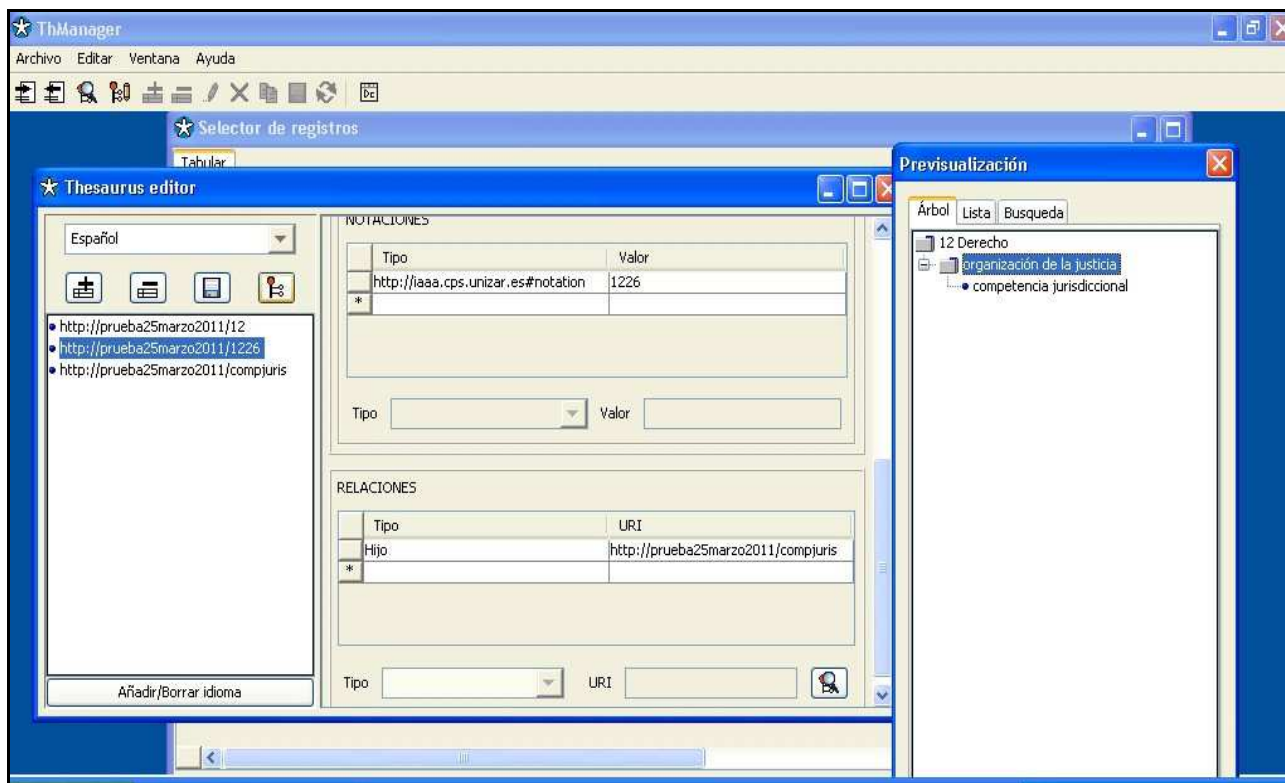
Figura 6. ThManager.
