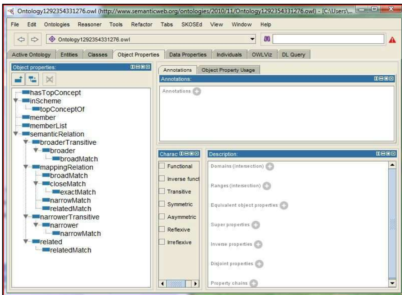
Figura 4. SKOSEd.
