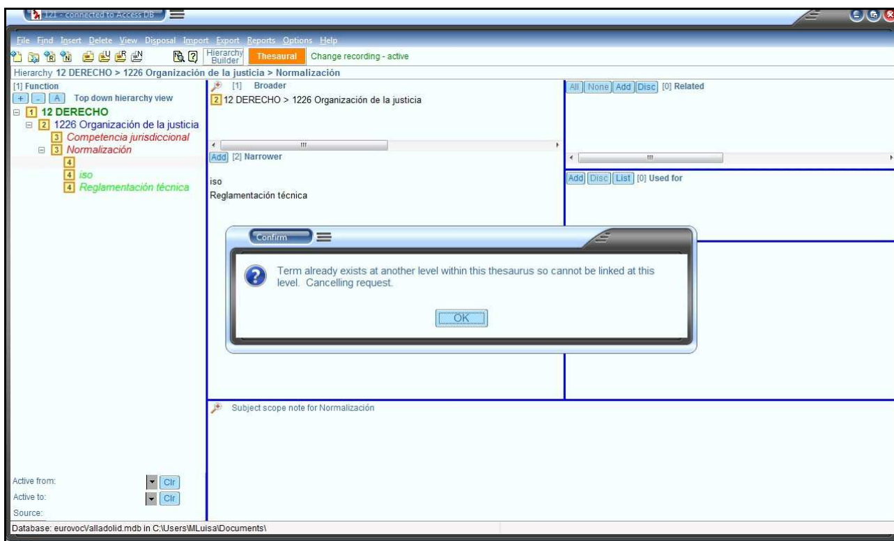
Figura 2. One-2-One.
