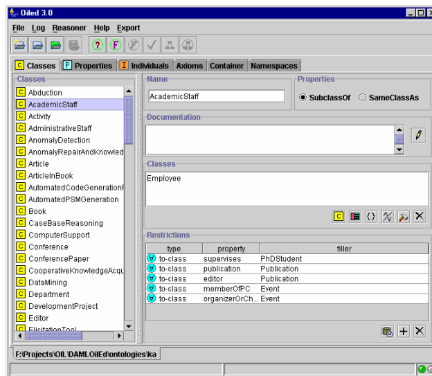
Fig. 4. Editor OilEd 3.0
