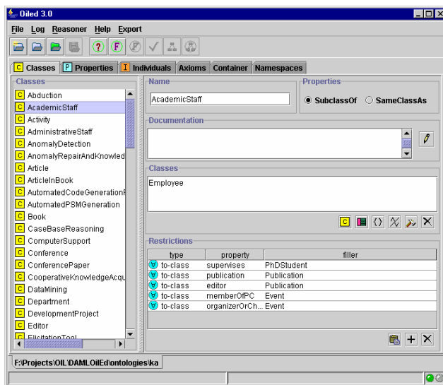
Fig. 4. Editor OilEd 3.0
